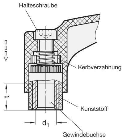
ELESA Original design ERS.
