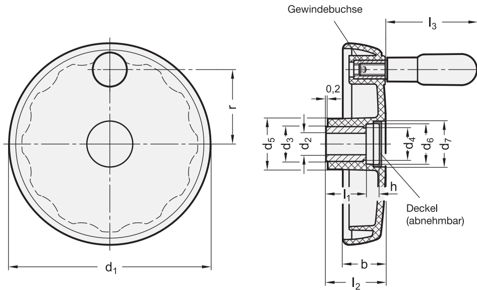
ELESA Original design VDS / VDS+i
