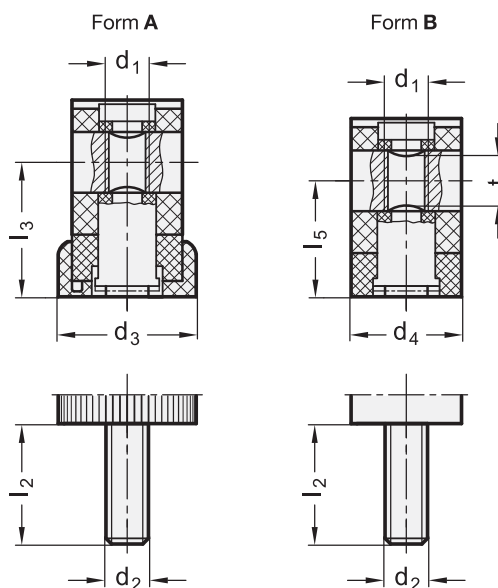
ELESA original design LAC / LAC-R
