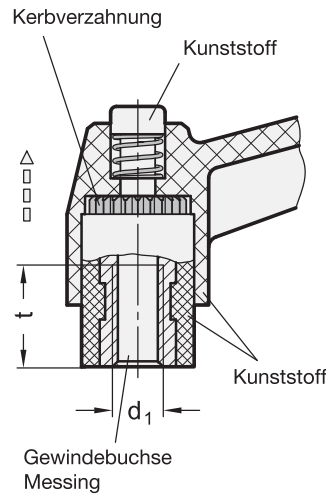
ELESA Original design MRX.
