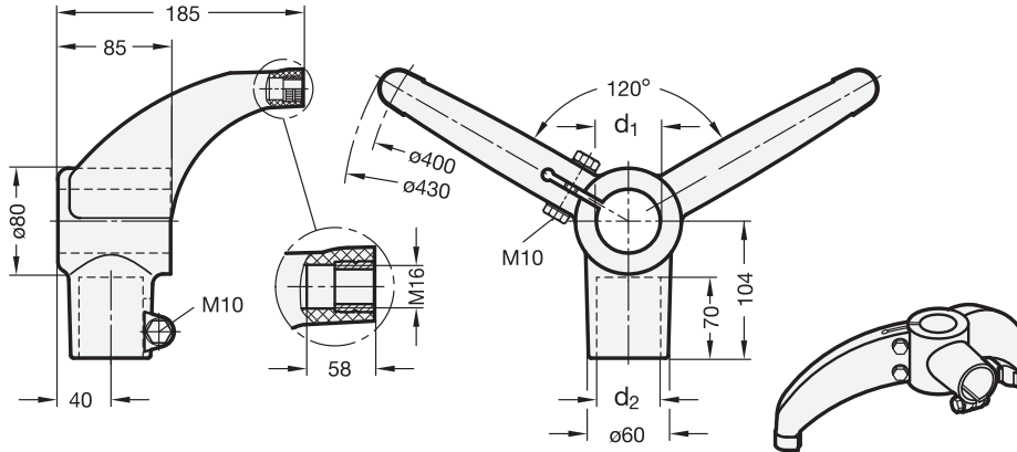
ELESA Original design BAG2-120
