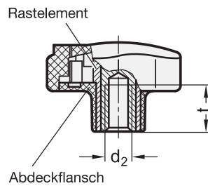
Schlüssel Form CSN
