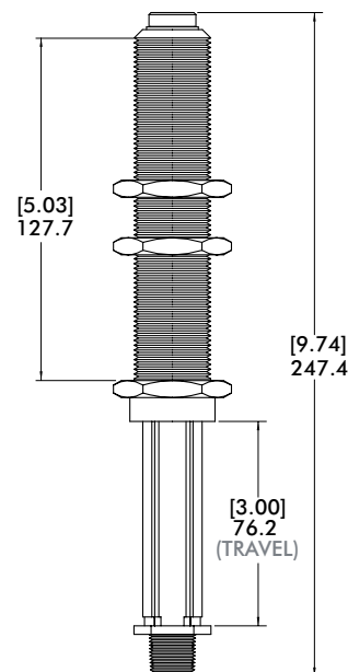
CPI-RCM-150-U14-NR Shown with CPI-SAP-30
