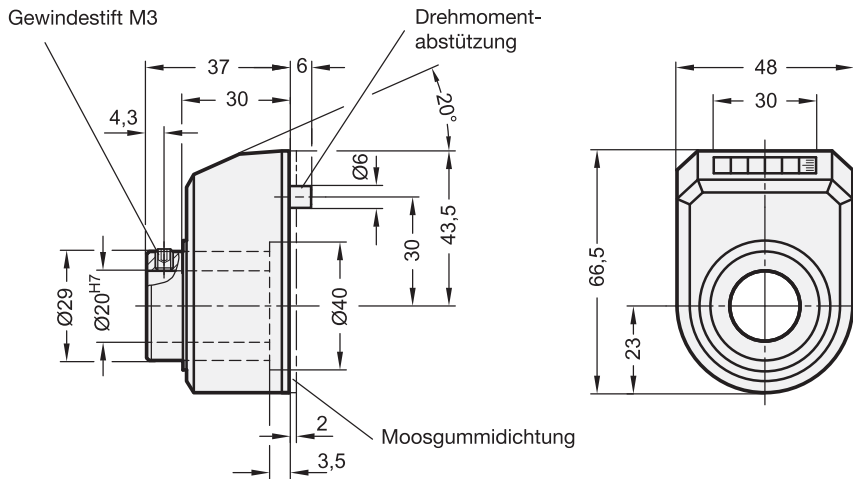
ELESA Original design DD52R
