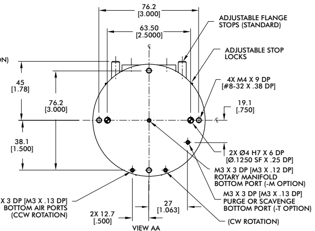
PLEASE NOTE: THE ONLY FEATURES THAT ARE NOT DIRECTLY RETROFITTABLE TO THE RR-26 IS THE DIFFERENT SENSORS & SENSOR MOUNTING KIT.
