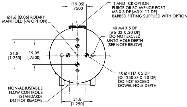
UNIT SHOWN IN 0° POSITION ROTATED FULLY CW
