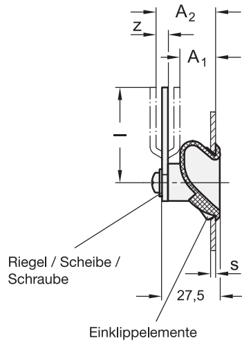
ELESA original design PR-CH / LPR
