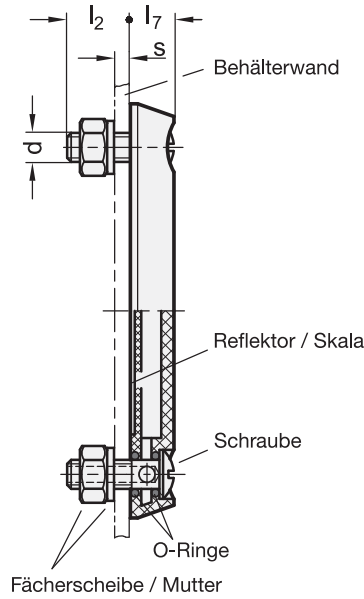
ELESA Original design HCX./HCX-SST
