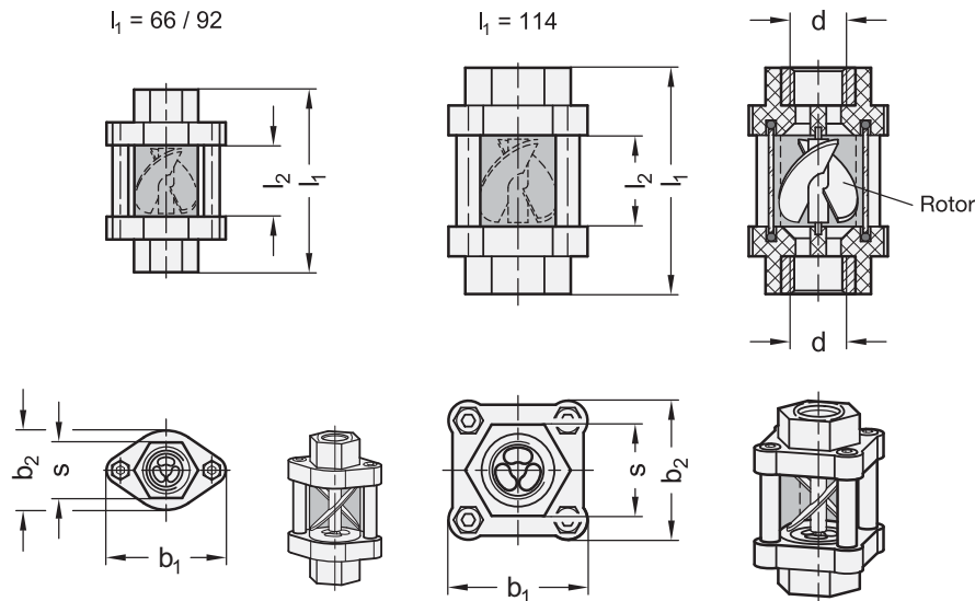
ELESA Original design HVF
