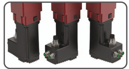
Motor connection positions can be rotated in 90° increments
