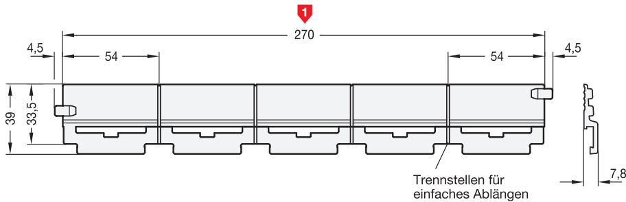
ELESA original design RLT-CE
