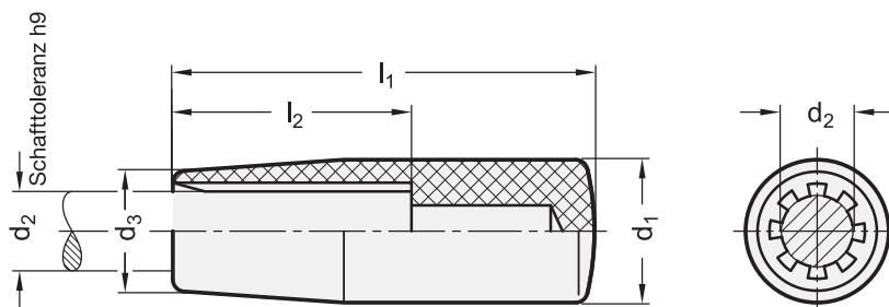
ELESA Original design I.580 N
