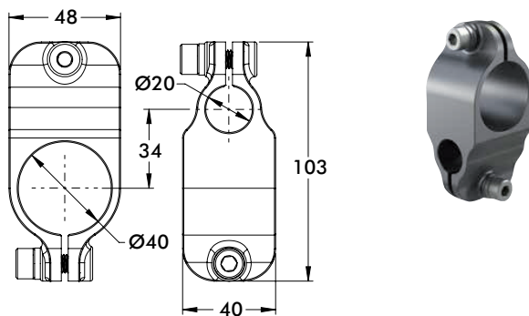
Ø40mm to Ø20mm Cross Clamp
