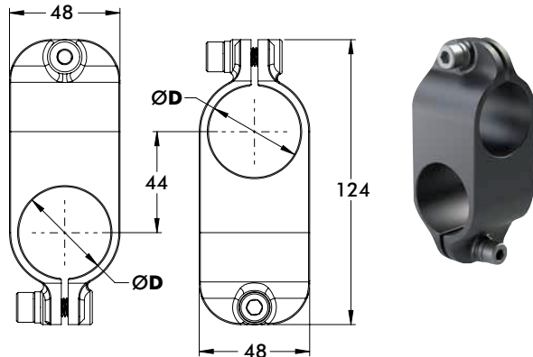
Ø40mm/1.50 in to Ø40mm/1.50 in Cross Clamp
