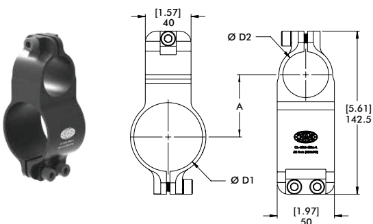
Ø60mm/2.50 in to Ø40mm/1.50 in Cross Clamp
