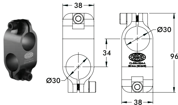
Ø30mm to Ø30mm Cross Clamp
