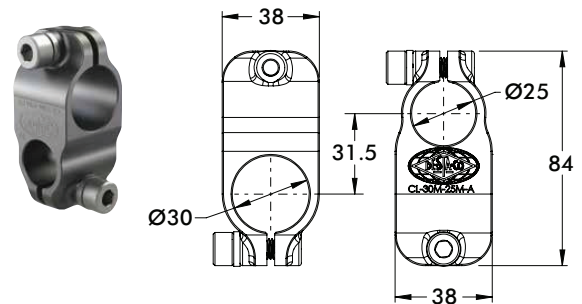
Ø30mm to Ø25mm Cross Clamp
