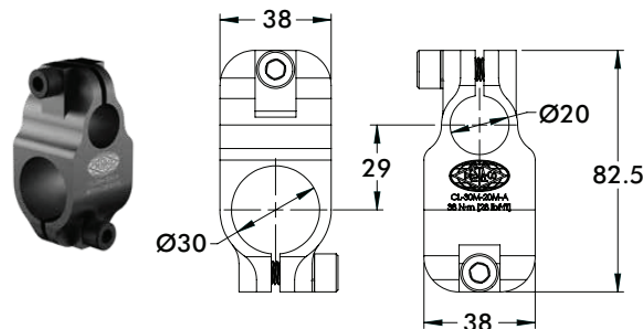
Ø30mm to Ø20mm Cross Clamp
