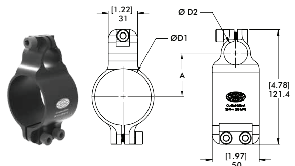
Ø60mm/2.50 in to Ø25mm/1.00 in Cross Clamp
