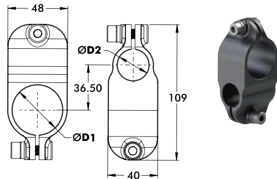
Ø40mm/1.50 in to Ø25mm/1.00 in Cross Clamp
