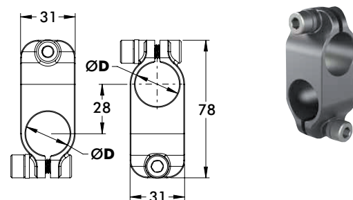
Ø25mm/1.00 in to Ø25mm/1.00 in Cross Clamp
