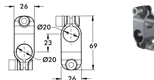
Ø20mm to Ø20mm Cross Clamp
