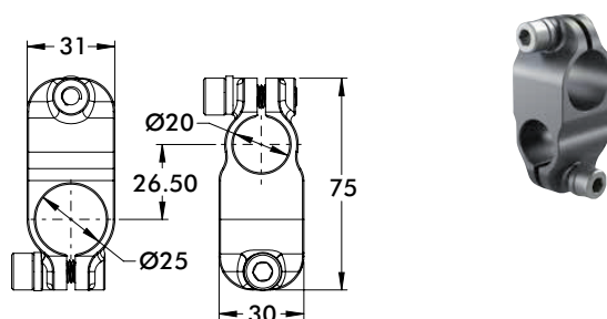
Ø25mm to Ø20mm Cross Clamp
