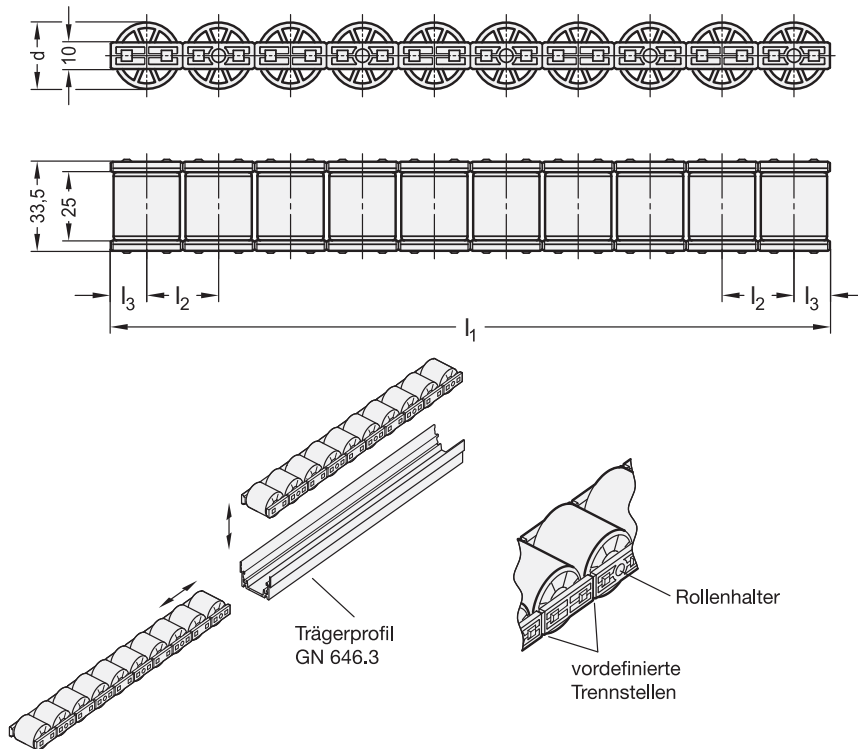
ELESA original design RLT-U
